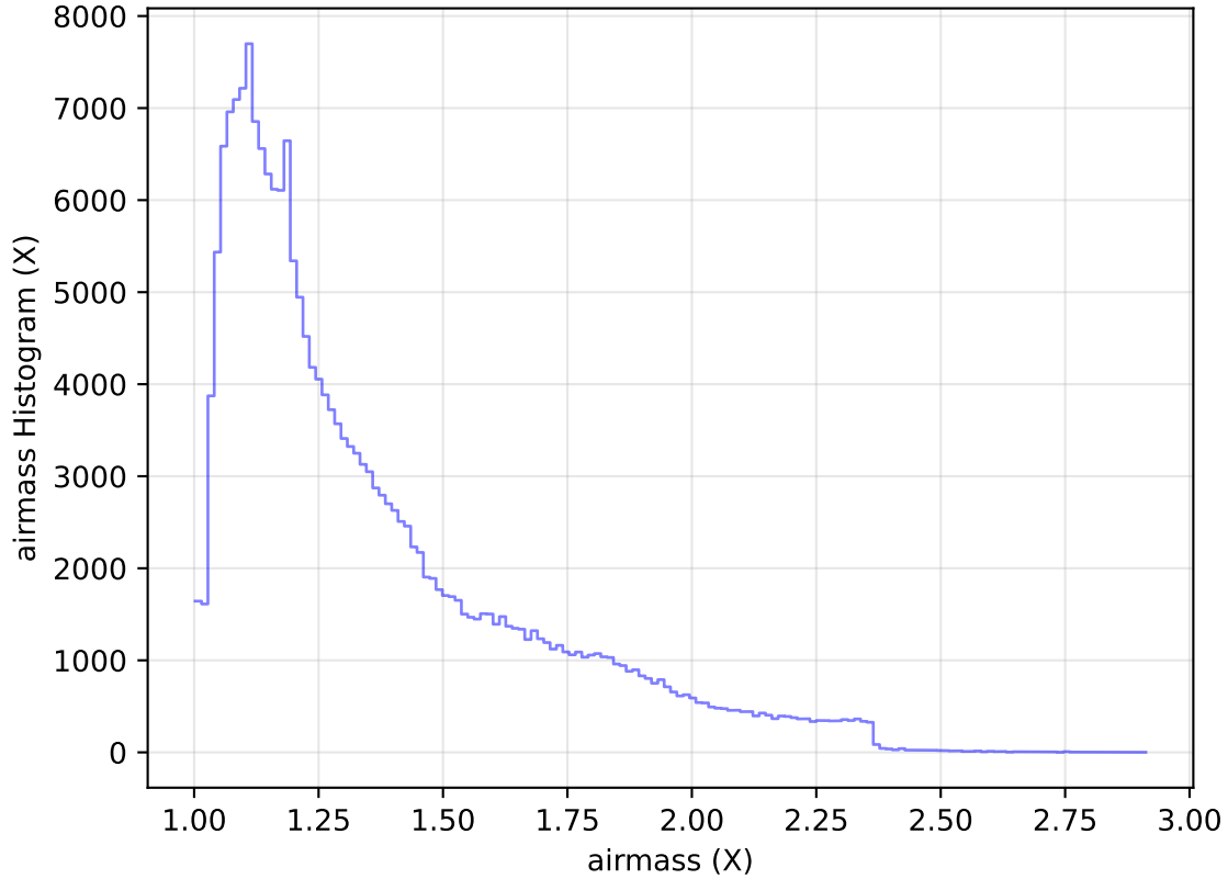
too_elab_heavy_r128_d3_ugrizy_v3.4_10yrs WFD g band: airmass Histogram
