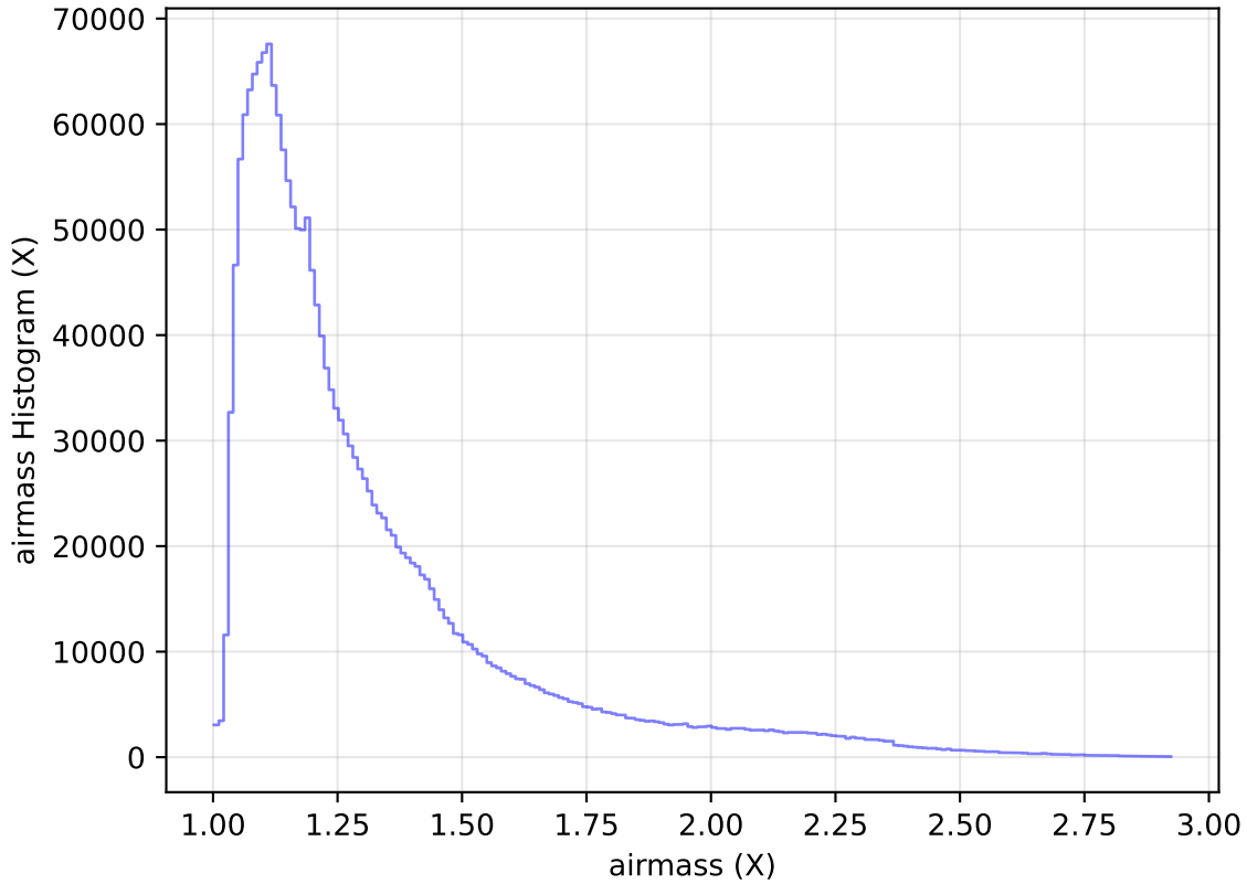
too_elab_heavy_r128_d3_ugrizy_v3.4_10yrs WFD all bands: airmass Histogram
