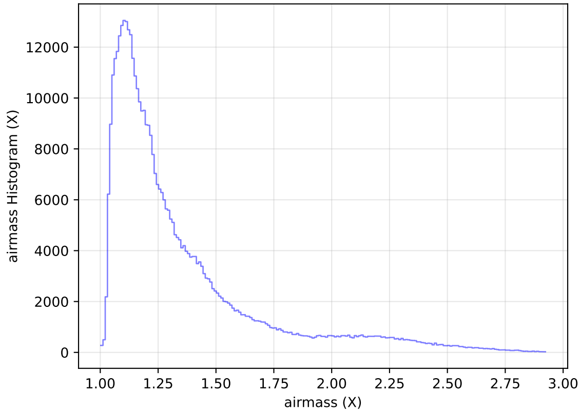
too_elab_heavy_r128_d3_ugrizy_v3.4_10yrs All sky z band: airmass Histogram
