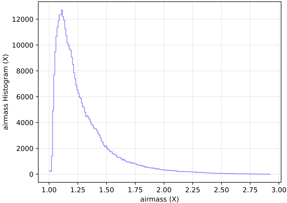
too_elab_heavy_r128_d3_ugrizy_v3.4_10yrs All sky y band: airmass Histogram
