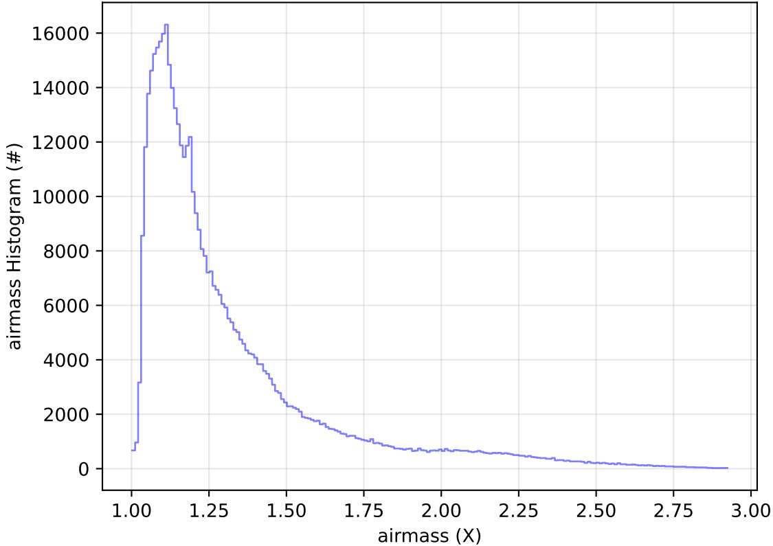
too_elab_heavy_r128_d3_ugrizy_v3.4_10yrs All sky i band: airmass Histogram
