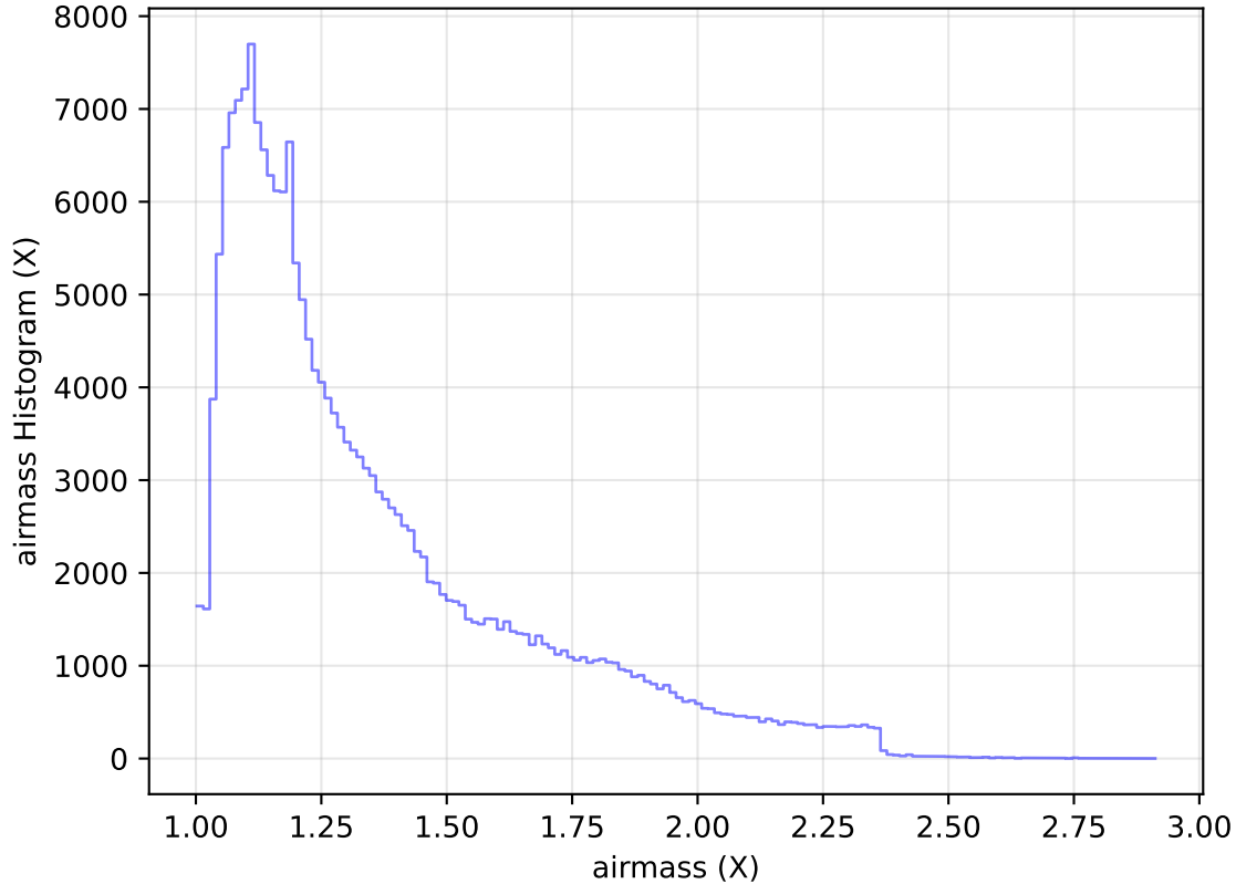
too_elab_heavy_r128_d3_ugrizy_v3.4_10yrs All sky g band: airmass Histogram
