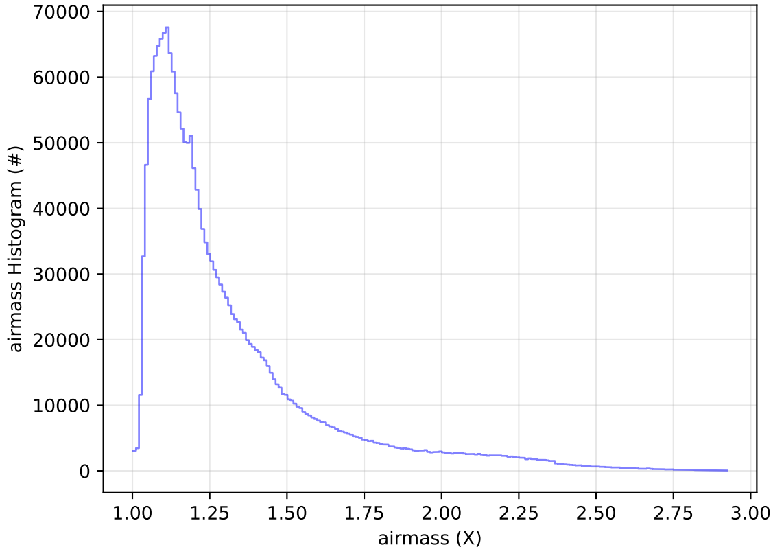
too_elab_heavy_r128_d3_ugrizy_v3.4_10yrs All sky all bands: airmass Histogram
