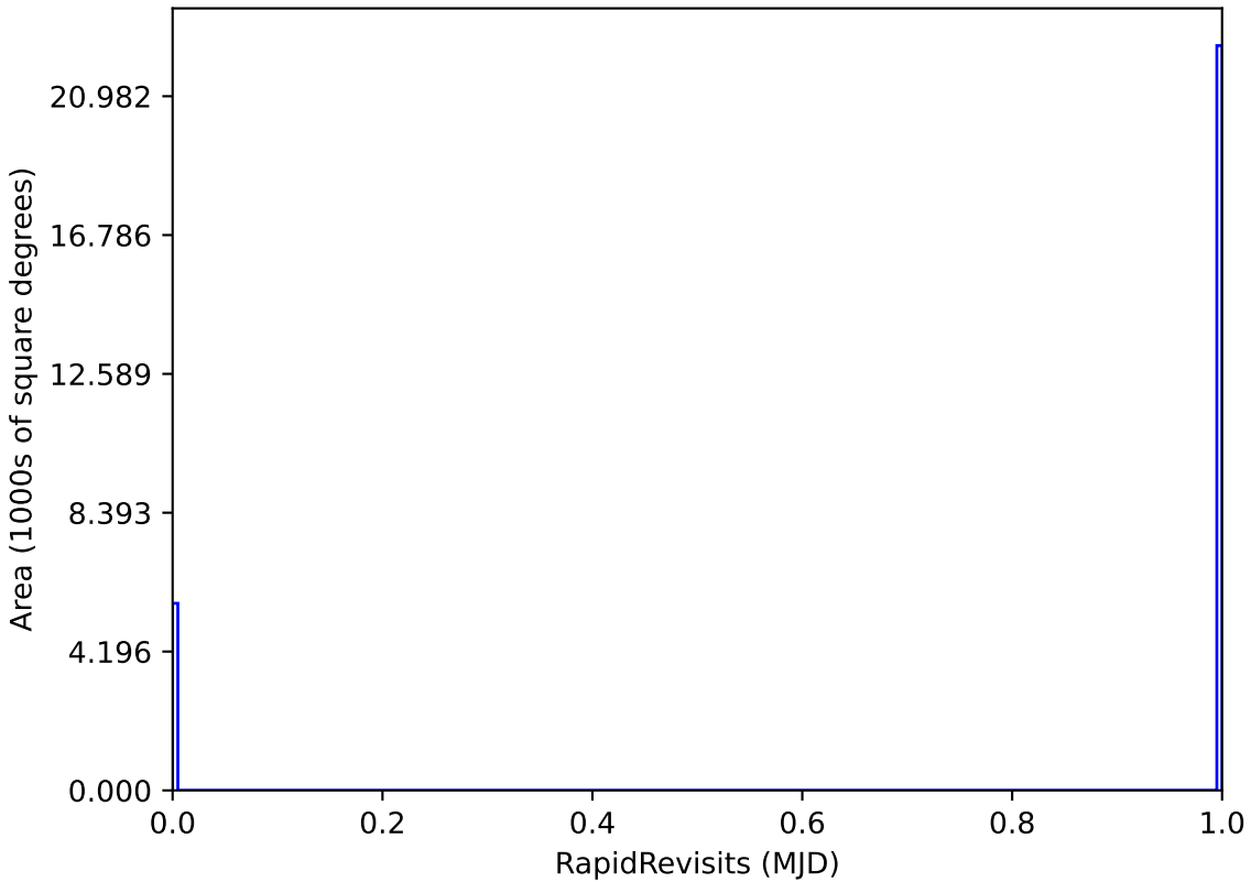
too_elab_heavy_r128_d3_ugrizy_v3.4_10yrs All sky: RapidRevisits
