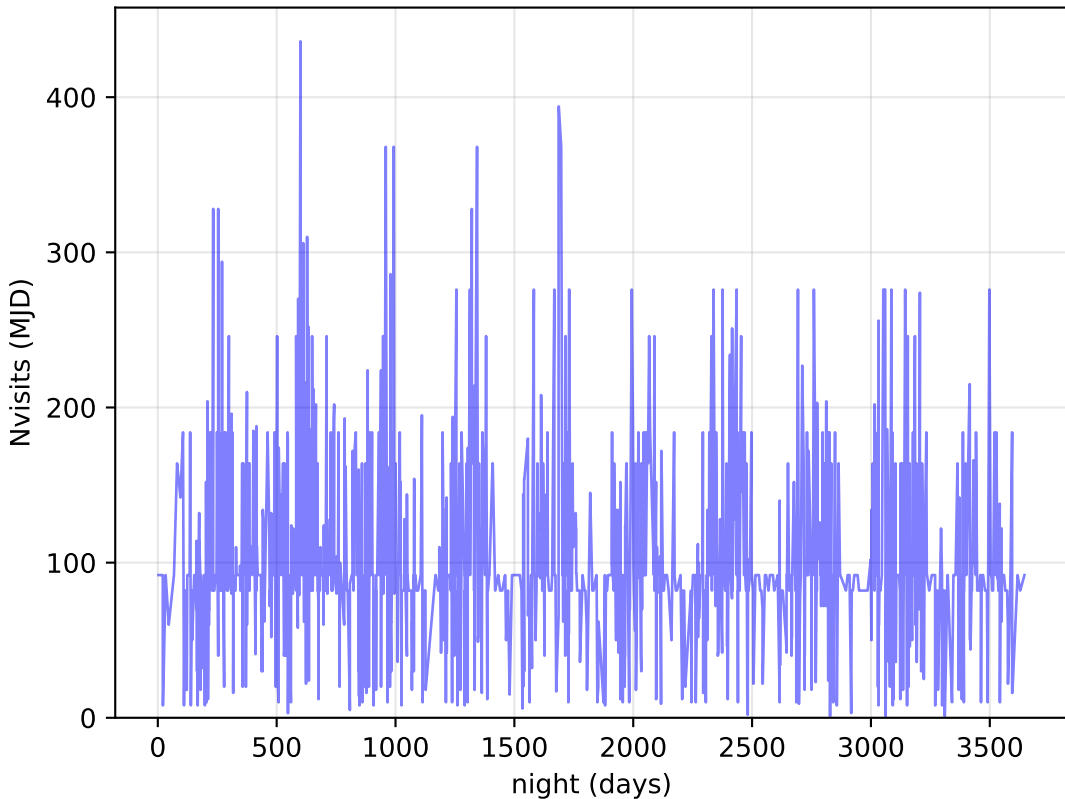
too_elab_heavy_r128_d3_ugrizy_v3.4_10yrs DDF: Nvisits
