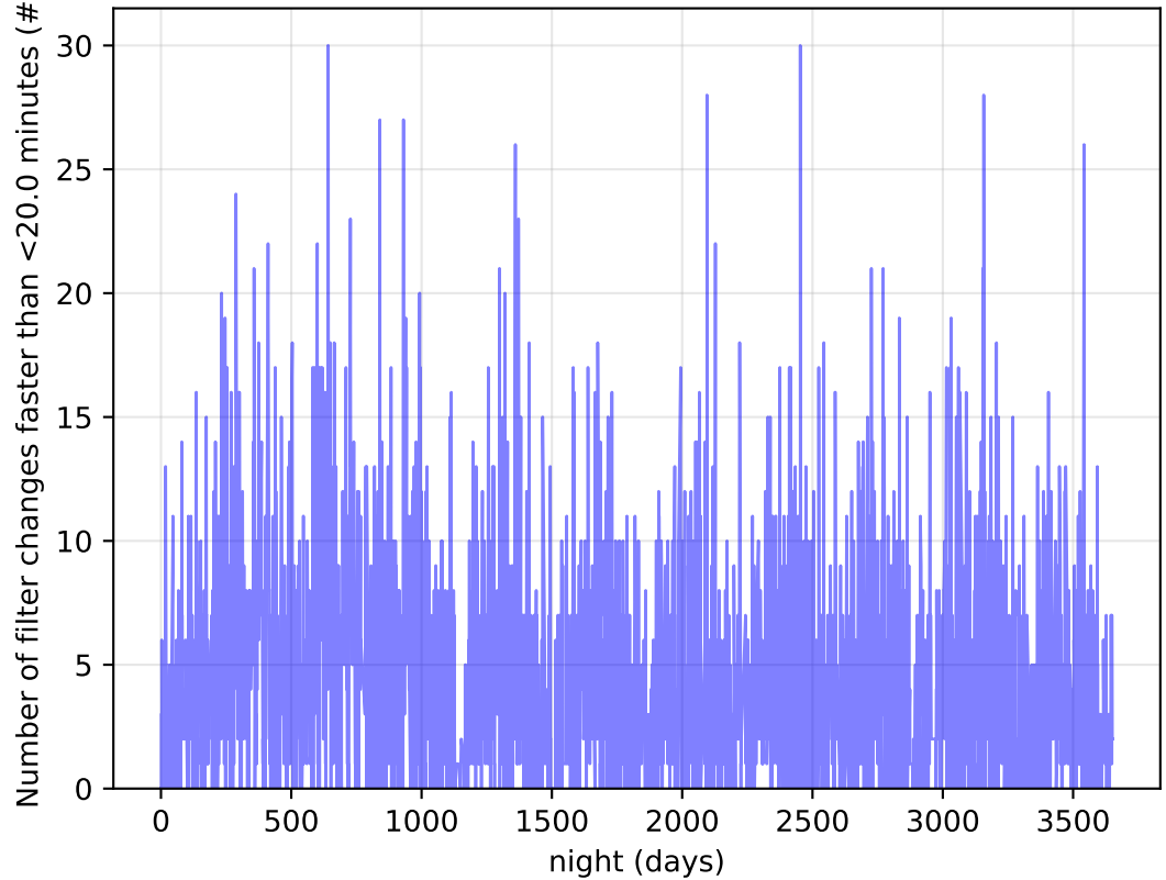
too_elab_heavy_r128_d3_ugrizy_v3.4_10yrs Per Night: Number of filter changes faster than <20.0 minutes
