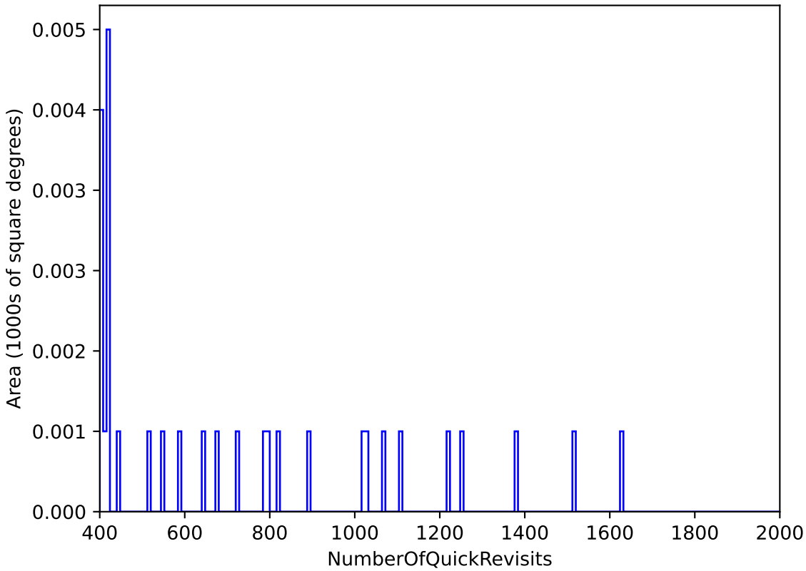
too_elab_heavy_r128_d3_ugrizy_v3.4_10yrs All sky: NumberOfQuickRevisits
