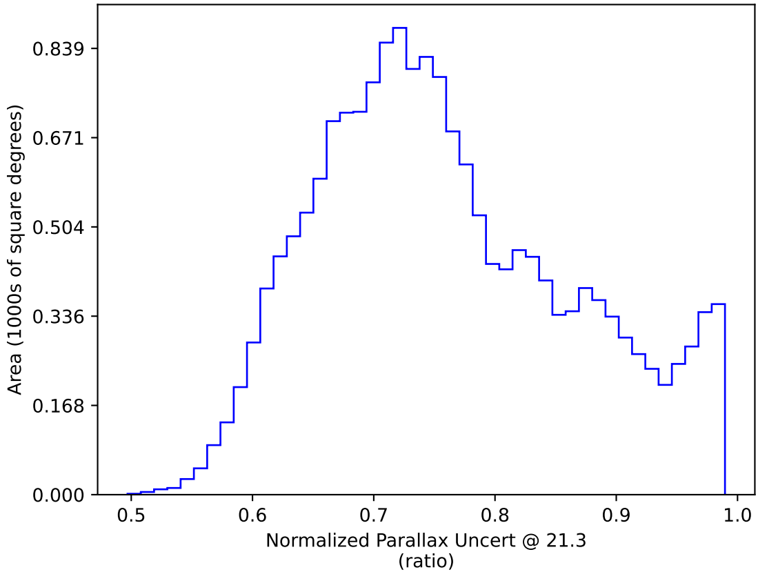
too_elab_heavy_r128_d3_ugrizy_v3.4_10yrs WFD y band only: Normalized Parallax Uncert @ 21.3
