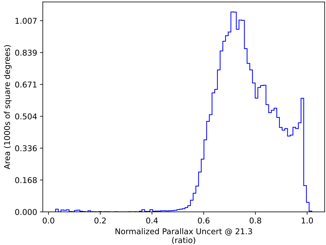
too_elab_heavy_r128_d3_ugrizy_v3.4_10yrs All sky y band only: Normalized Parallax Uncert @ 21.3
