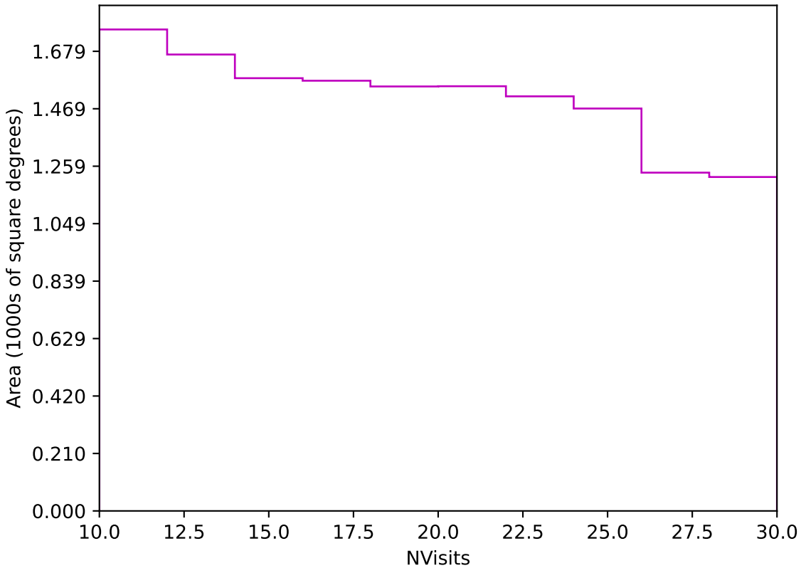
too_elab_heavy_r128_d3_ugrizy_v3.4_10yrs Yr 3-4 z band: NVisits
