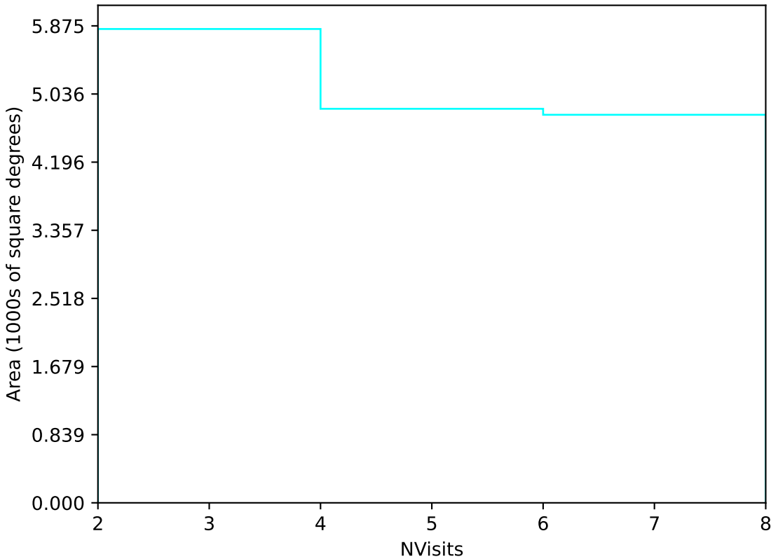
too_elab_heavy_r128_d3_ugrizy_v3.4_10yrs Yr 3-4 u band: NVisits
