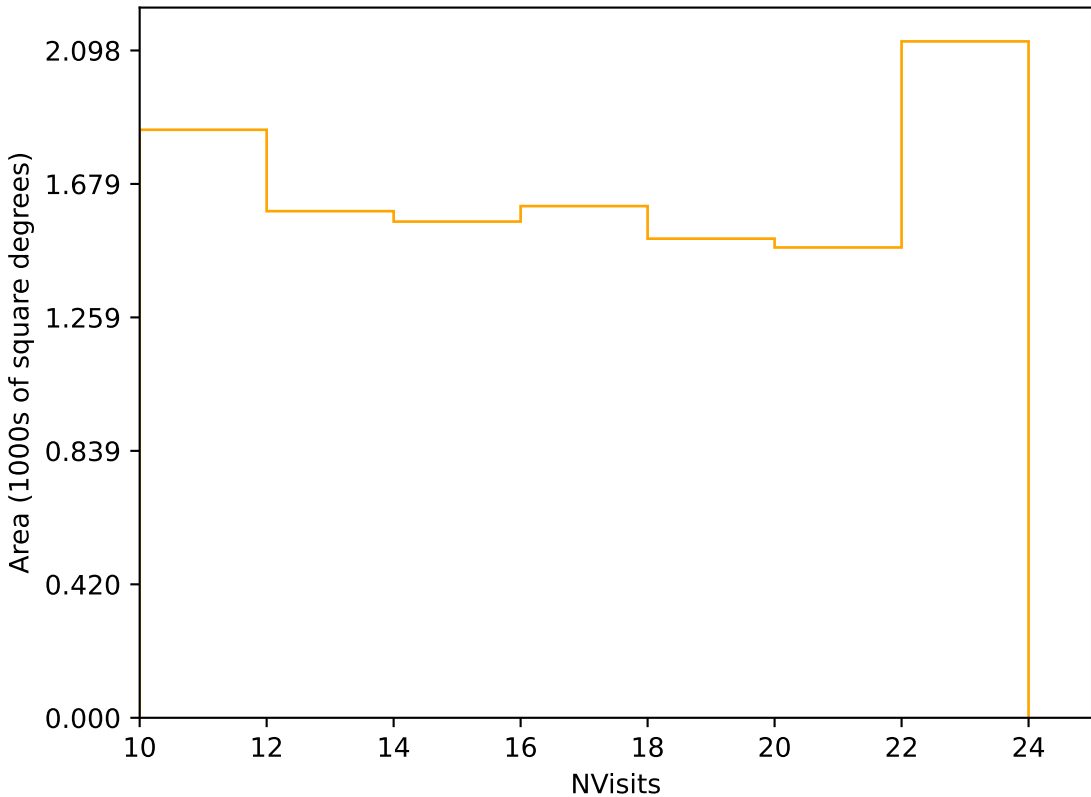
too_elab_heavy_r128_d3_ugrizy_v3.4_10yrs Yr 3-4 r band: NVisits
