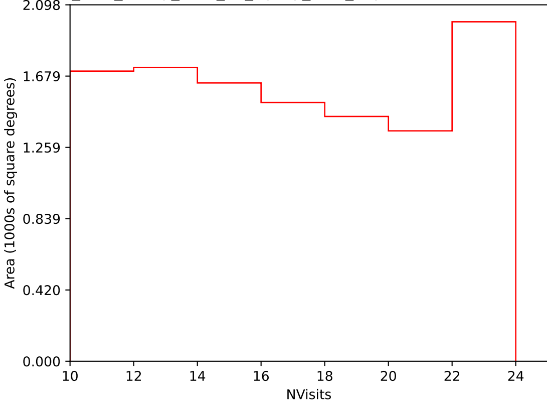
too_elab_heavy_r128_d3_ugrizy_v3.4_10yrs Yr 3-4 i band: NVisits
