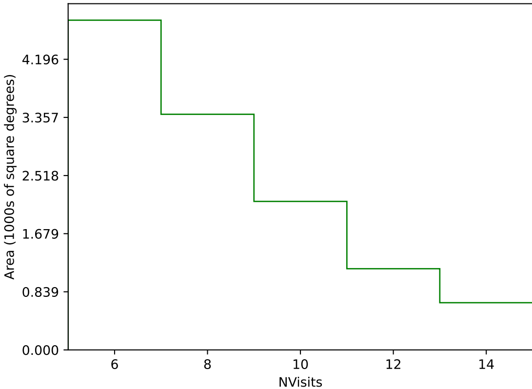
too_elab_heavy_r128_d3_ugrizy_v3.4_10yrs Yr 3-4 g band: NVisits
