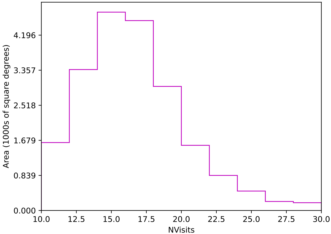
too_elab_heavy_r128_d3_ugrizy_v3.4_10yrs Yr 1 z band: NVisits
