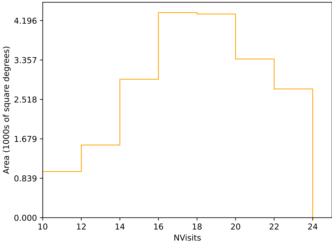
too_elab_heavy_r128_d3_ugrizy_v3.4_10yrs Yr 1 r band: NVisits
