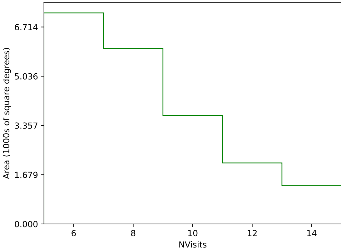
too_elab_heavy_r128_d3_ugrizy_v3.4_10yrs Yr 1 g band: NVisits
