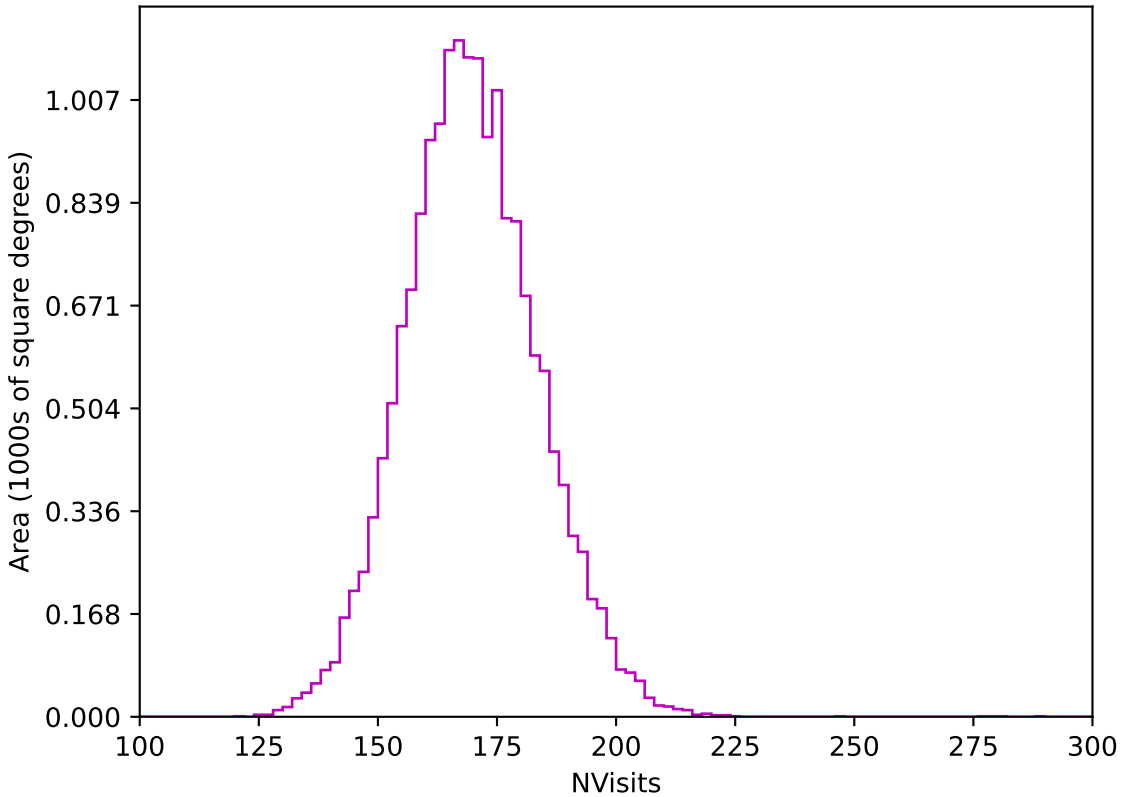
too_elab_heavy_r128_d3_ugrizy_v3.4_10yrs WFD z band: NVisits
