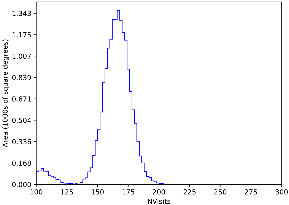
too_elab_heavy_r128_d3_ugrizy_v3.4_10yrs WFD y band: NVisits
