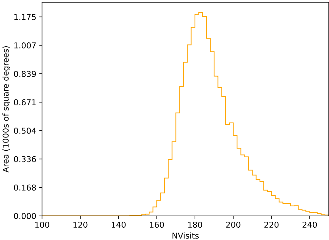
too_elab_heavy_r128_d3_ugrizy_v3.4_10yrs WFD r band: NVisits
