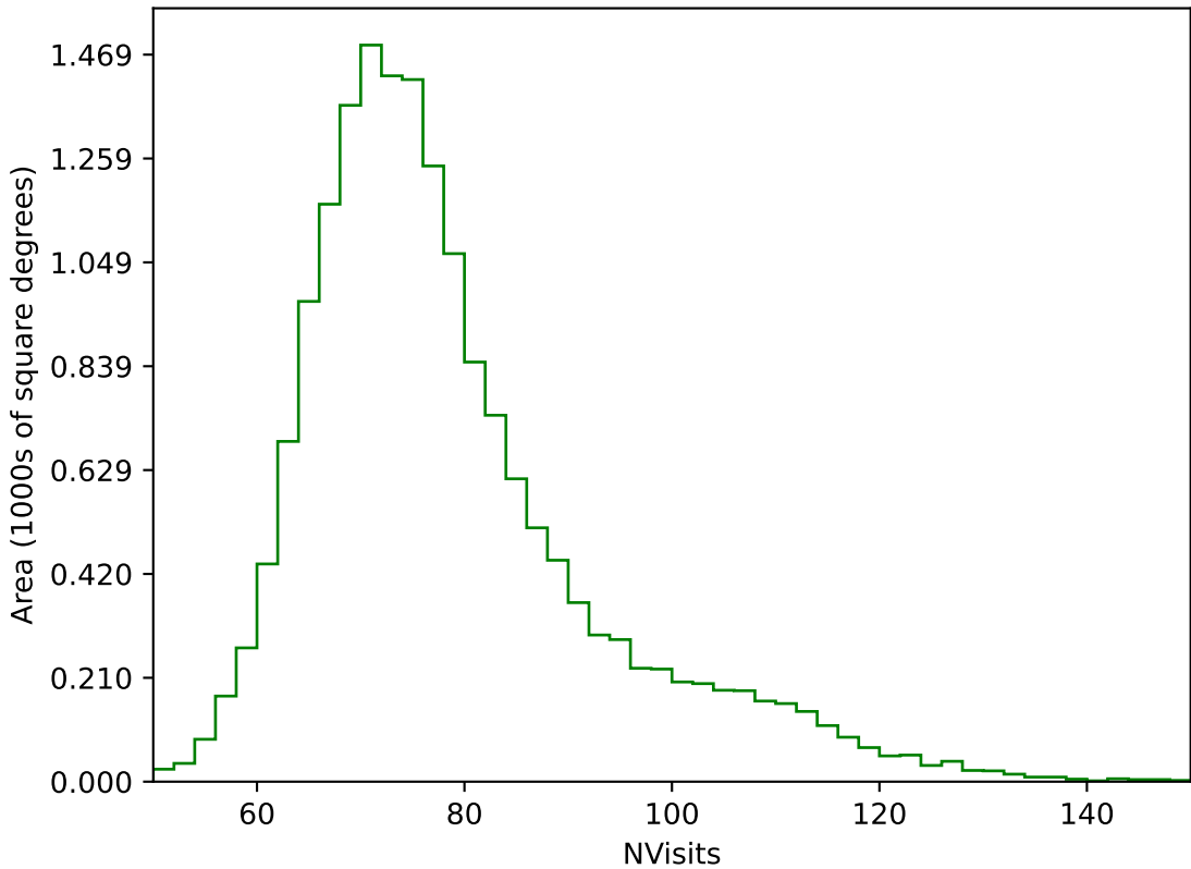
too_elab_heavy_r128_d3_ugrizy_v3.4_10yrs WFD g band: NVisits
