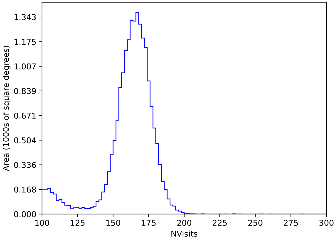
too_elab_heavy_r128_d3_ugrizy_v3.4_10yrs All sky y band: NVisits
