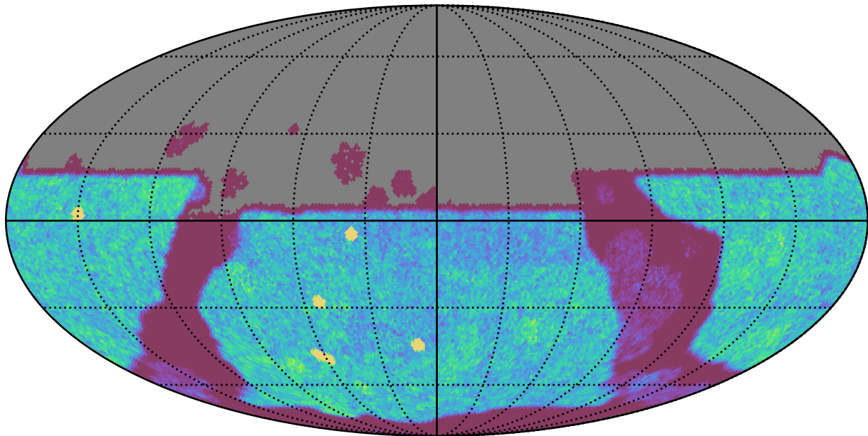
too_elab_heavy_r128_d3_ugrizy_v3.4_10yrs All sky u band: NVisits
