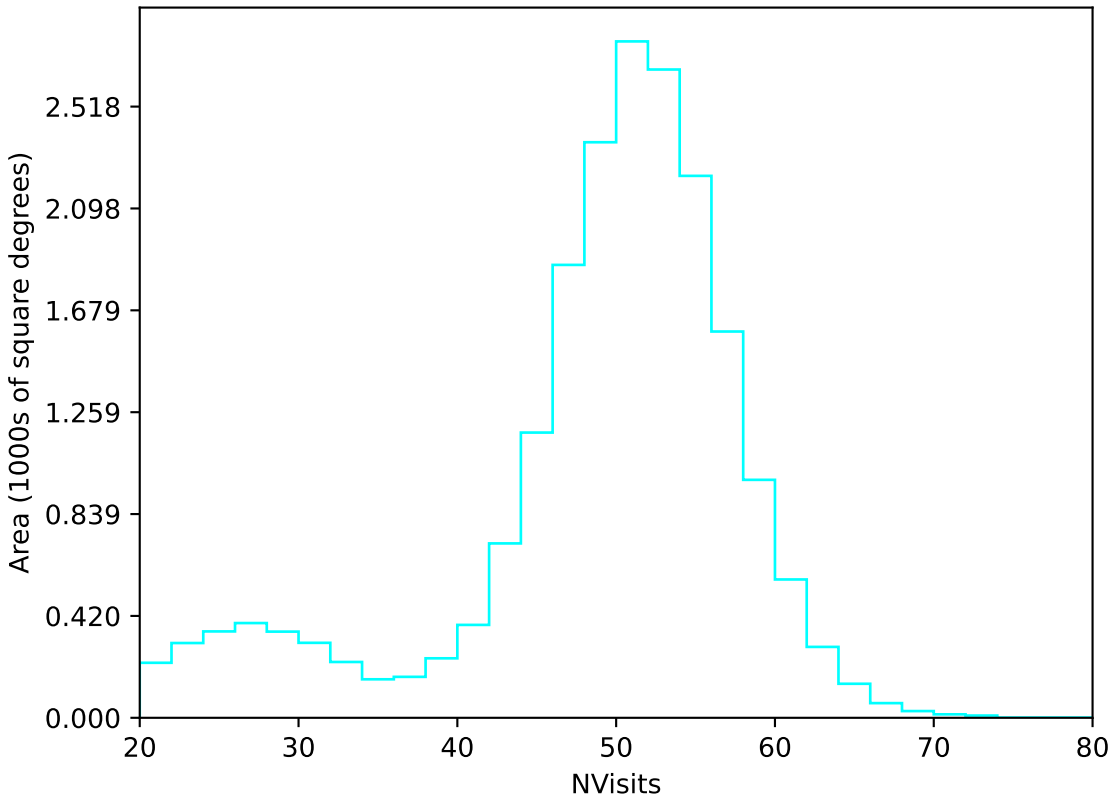
too_elab_heavy_r128_d3_ugrizy_v3.4_10yrs All sky u band: NVisits
