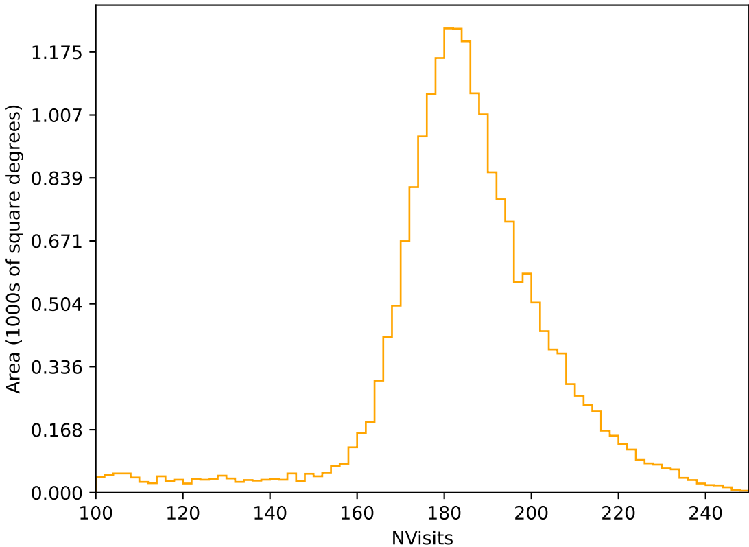
too_elab_heavy_r128_d3_ugrizy_v3.4_10yrs All sky r band: NVisits
