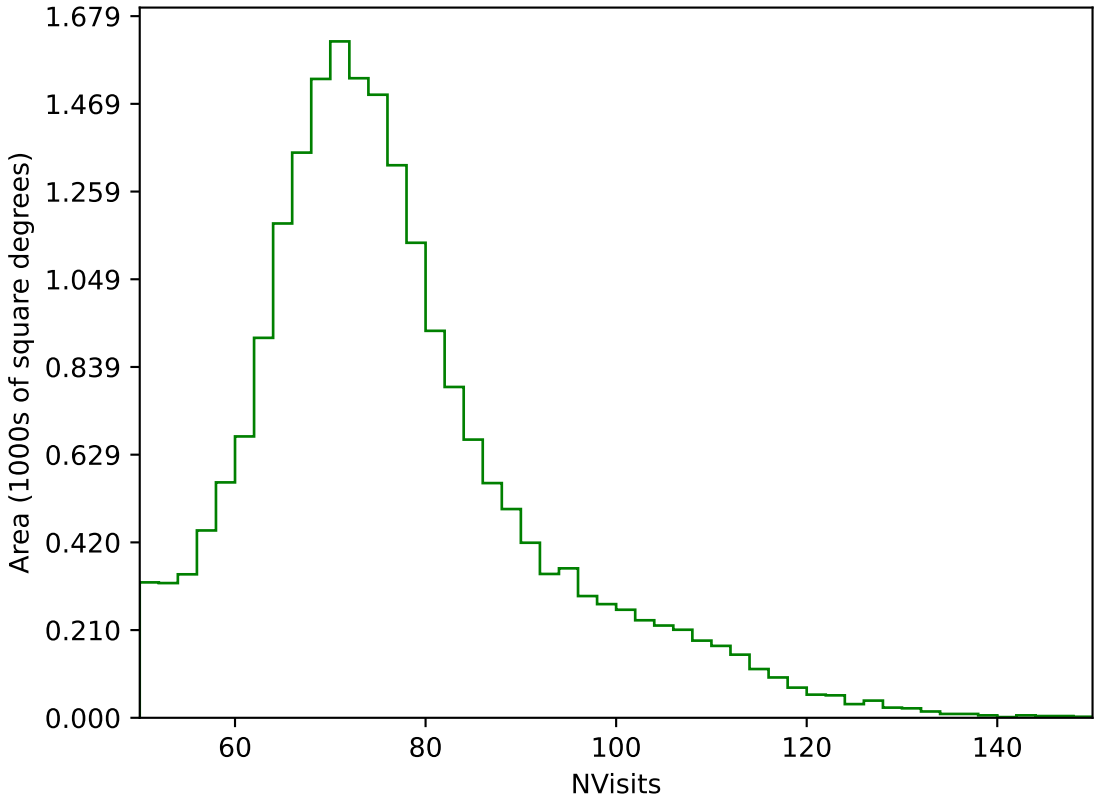
too_elab_heavy_r128_d3_ugrizy_v3.4_10yrs All sky g band: NVisits
