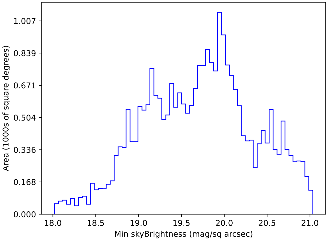
too_elab_heavy_r128_d3_ugrizy_v3.4_10yrs Yr 1 r band: Min skyBrightness
