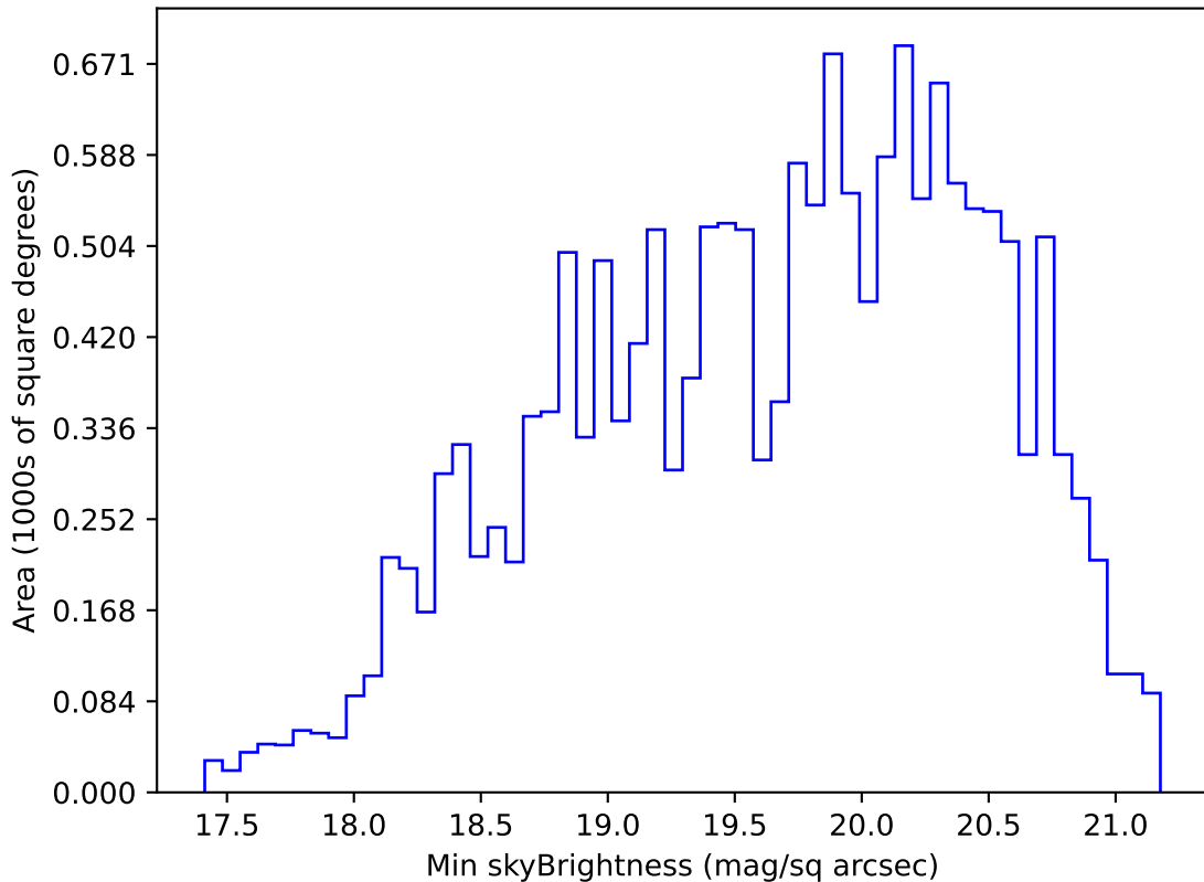
too_elab_heavy_r128_d3_ugrizy_v3.4_10yrs WFD g band: Min skyBrightness
