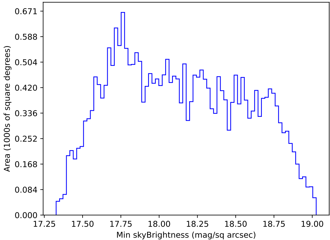
too_elab_heavy_r128_d3_ugrizy_v3.4_10yrs All sky i band: Min skyBrightness
