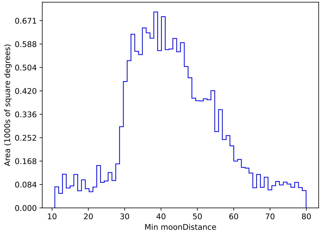
too_elab_heavy_r128_d3_ugrizy_v3.4_10yrs WFD g band: Min moonDistance
