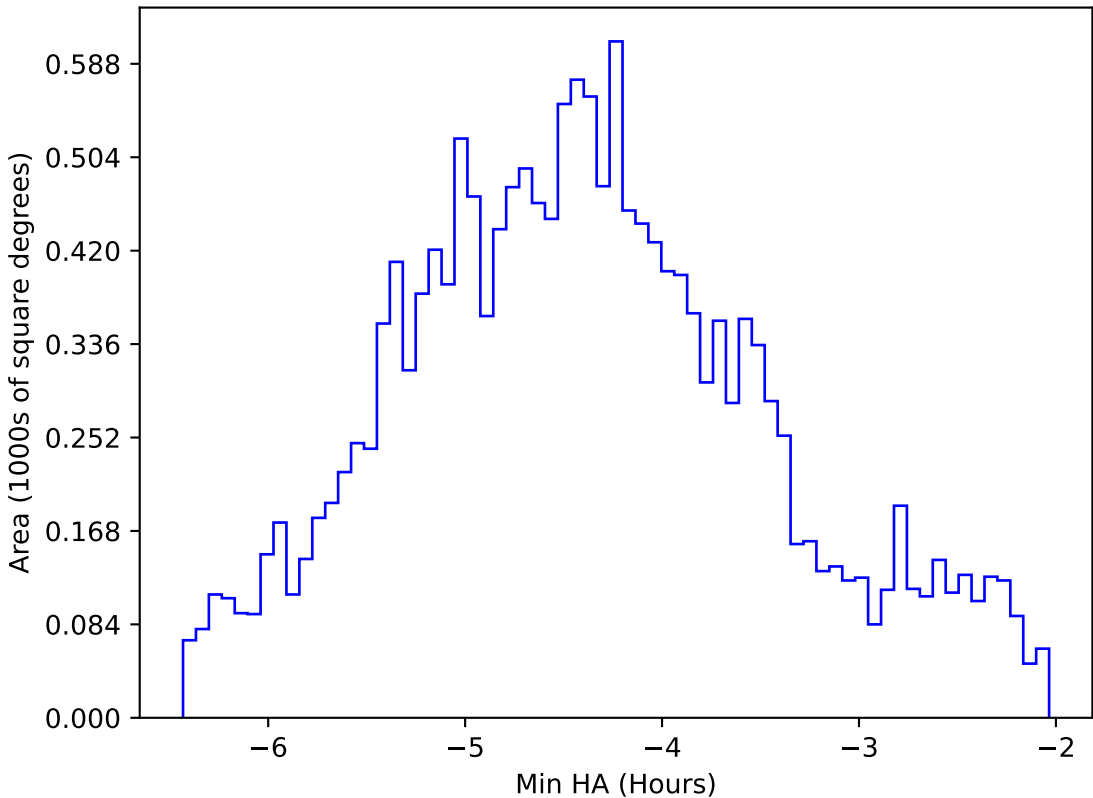
too_elab_heavy_r128_d3_ugrizy_v3.4_10yrs WFD z band: Min HA
