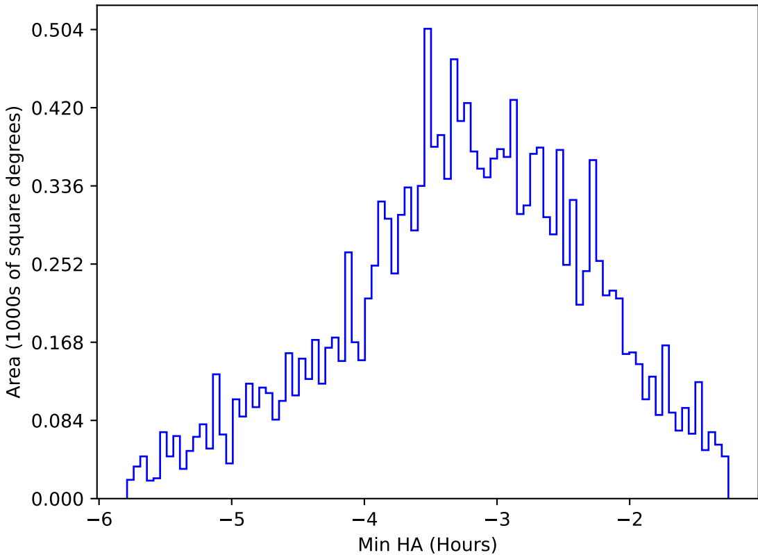
too_elab_heavy_r128_d3_ugrizy_v3.4_10yrs WFD u band: Min HA
