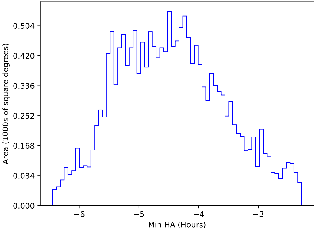
too_elab_heavy_r128_d3_ugrizy_v3.4_10yrs WFD r band: Min HA
