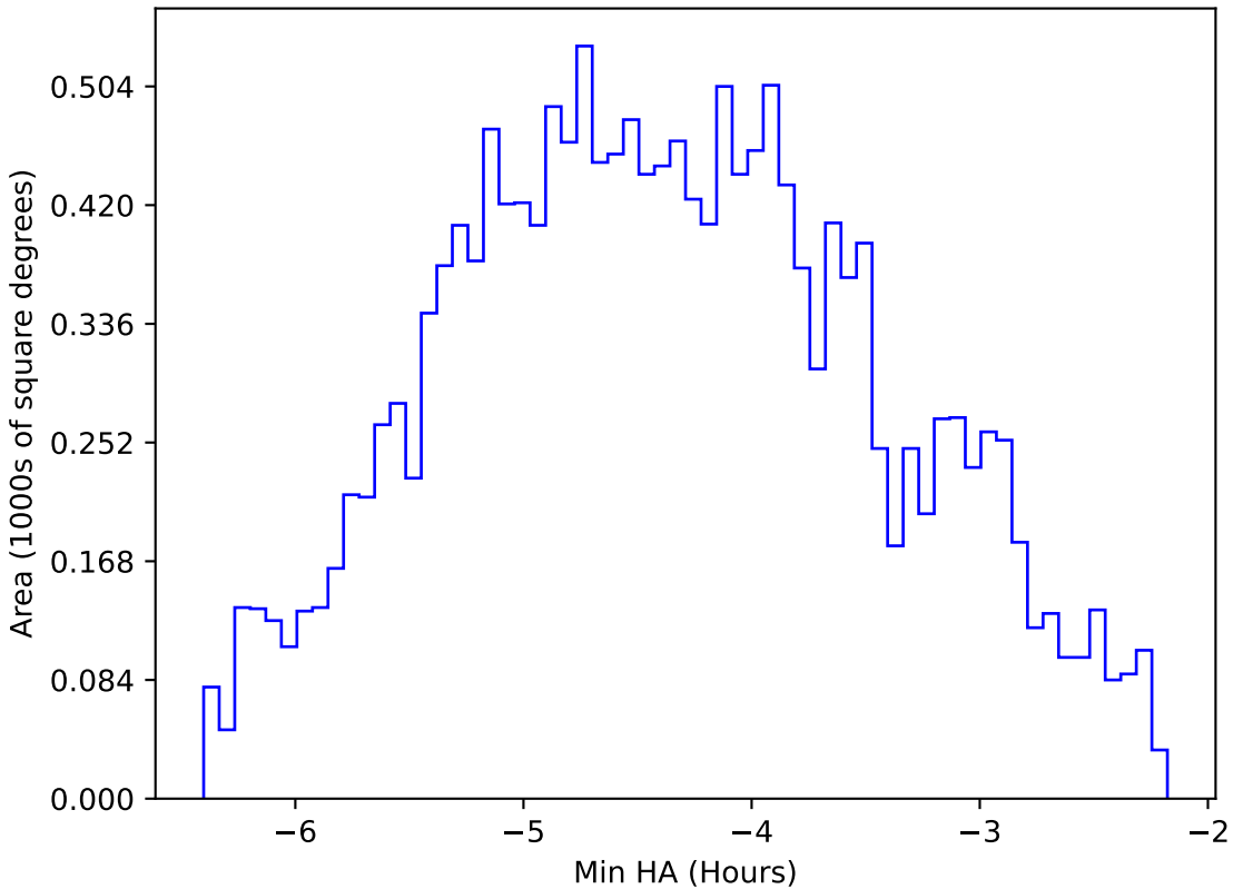
too_elab_heavy_r128_d3_ugrizy_v3.4_10yrs WFD i band: Min HA
