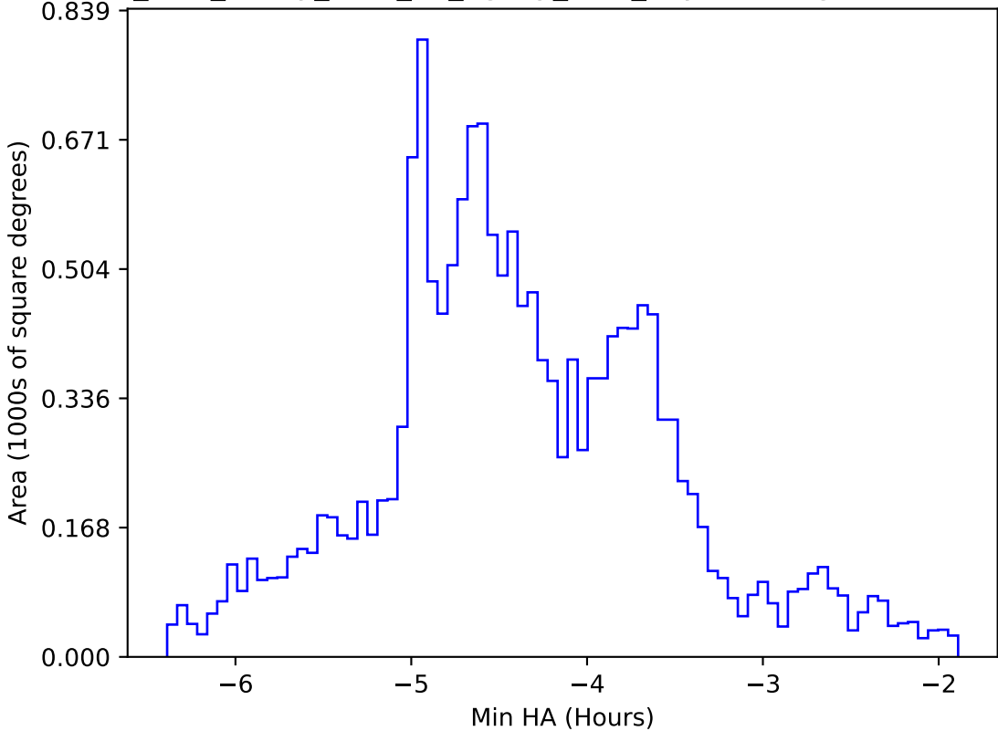
too_elab_heavy_r128_d3_ugrizy_v3.4_10yrs WFD g band: Min HA
