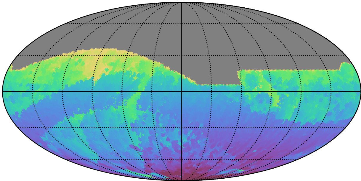
too_elab_heavy_r128_d3_ugrizy_v3.4_10yrs All sky r band: Min HA
