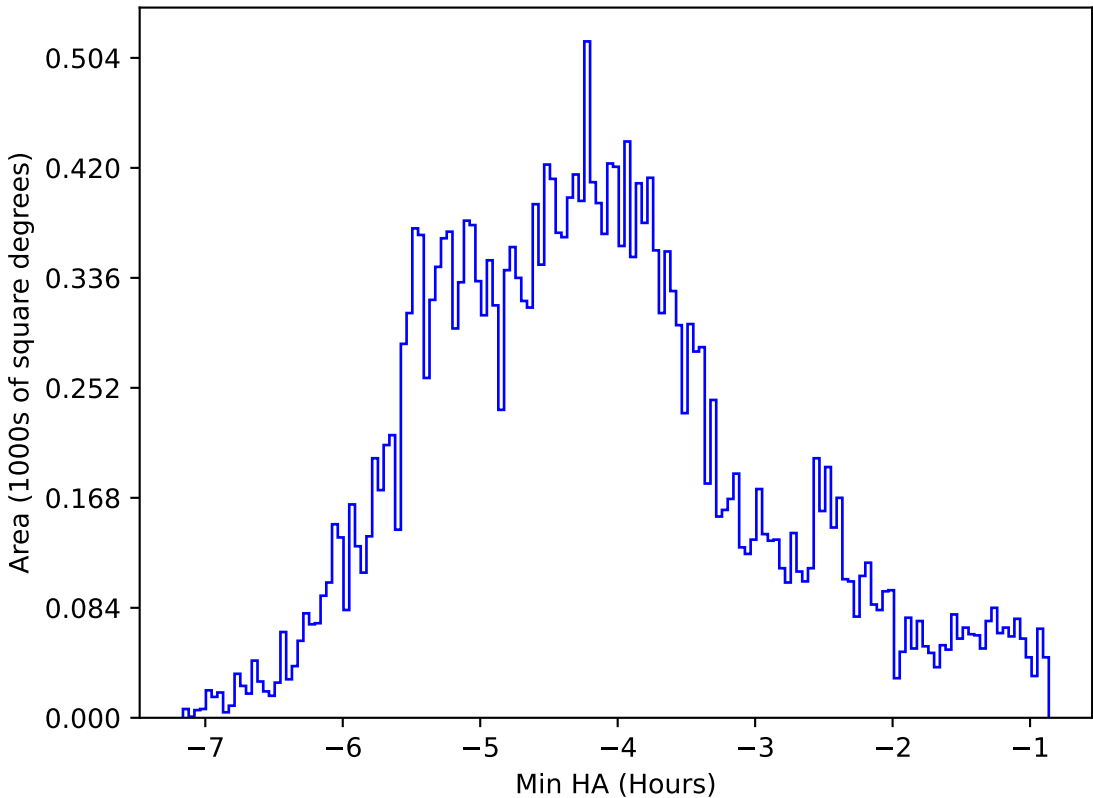
too_elab_heavy_r128_d3_ugrizy_v3.4_10yrs All sky r band: Min HA
