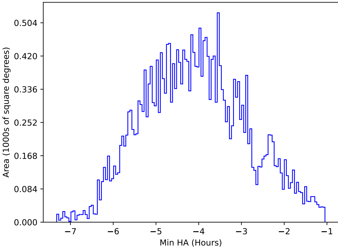
too_elab_heavy_r128_d3_ugrizy_v3.4_10yrs All sky i band: Min HA
