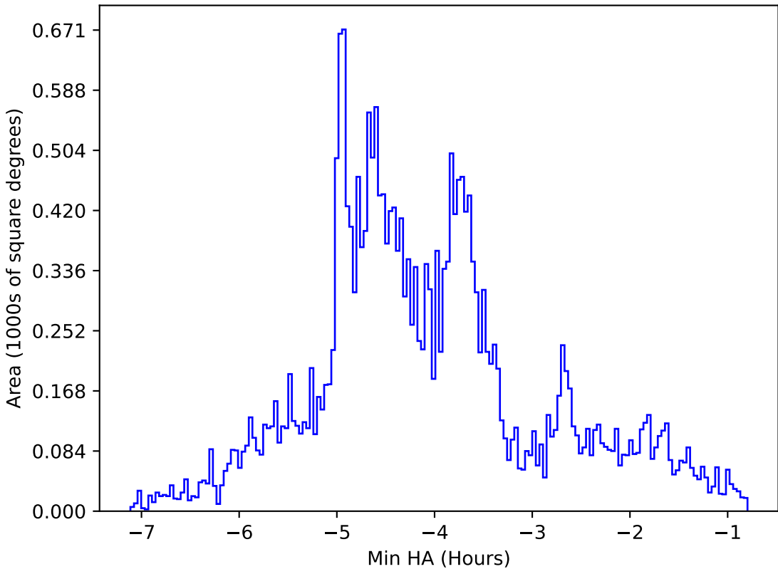
too_elab_heavy_r128_d3_ugrizy_v3.4_10yrs All sky g band: Min HA
