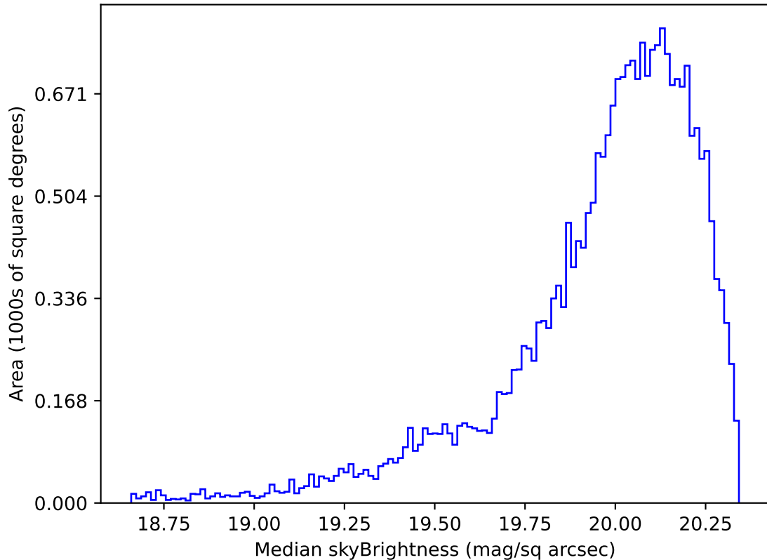
too_elab_heavy_r128_d3_ugrizy_v3.4_10yrs Yr 1 i band: Median skyBrightness
