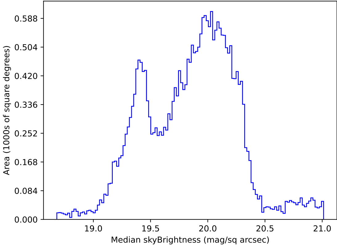
too_elab_heavy_r128_d3_ugrizy_v3.4_10yrs Yr 1 all bands: Median skyBrightness
