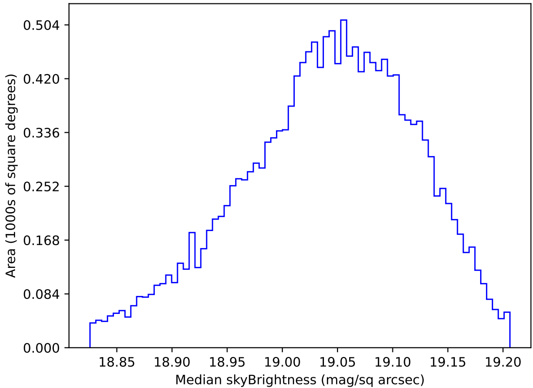
too_elab_heavy_r128_d3_ugrizy_v3.4_10yrs WFD z band: Median skyBrightness
