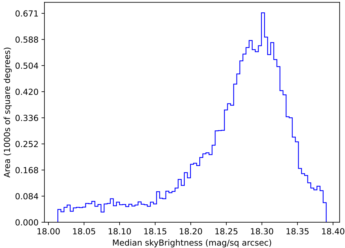
too_elab_heavy_r128_d3_ugrizy_v3.4_10yrs WFD y band: Median skyBrightness
