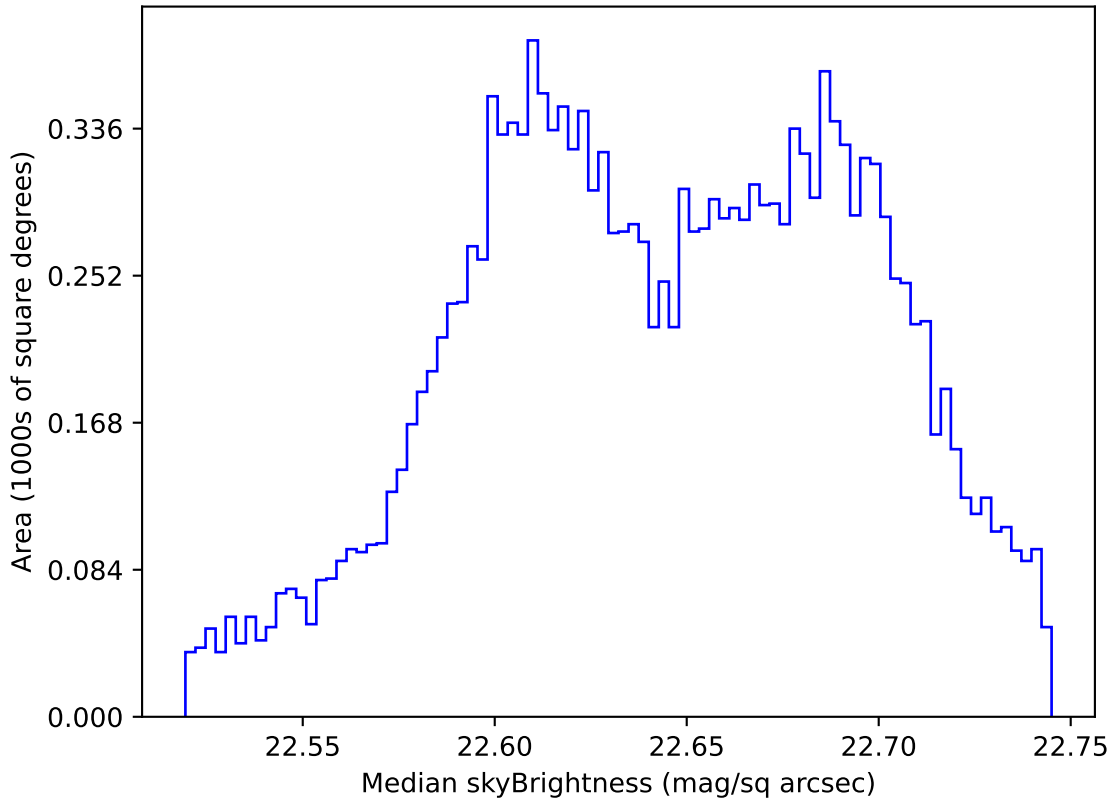
too_elab_heavy_r128_d3_ugrizy_v3.4_10yrs WFD u band: Median skyBrightness
