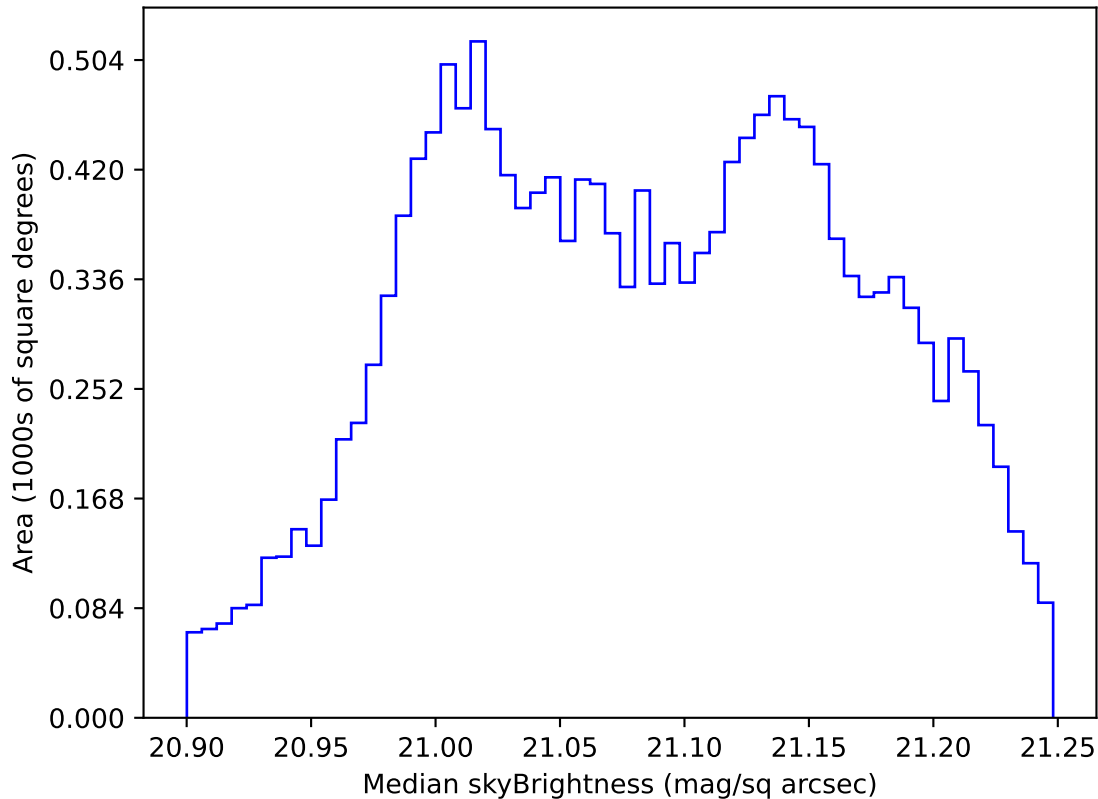
too_elab_heavy_r128_d3_ugrizy_v3.4_10yrs WFD r band: Median skyBrightness
