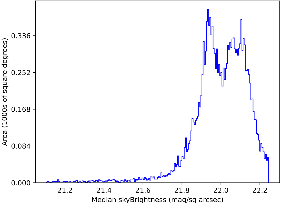
too_elab_heavy_r128_d3_ugrizy_v3.4_10yrs WFD g band: Median skyBrightness
